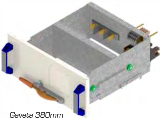
Gaveta 380mm
